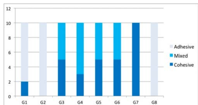
Figure 2 – Percentage (%) of the failure types during the micro shear bond strength testing (n = 10, per group)
