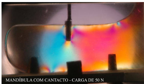
Figure 5c - Mandible with support and load of 50 N
